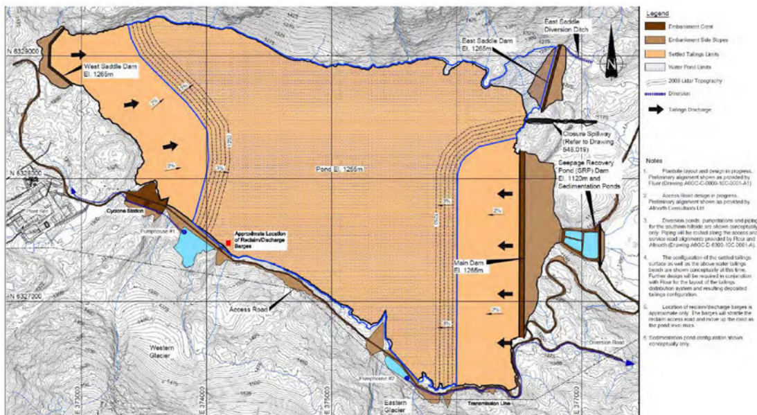
Figure 9 — Galore Creek Proposed Tailings Impoundment Layout
