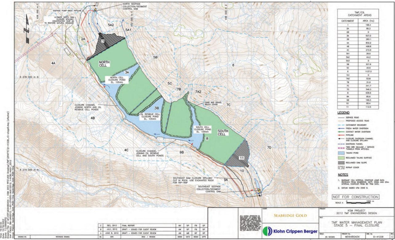
Figure 5 — KSM Final Closure Configuration
