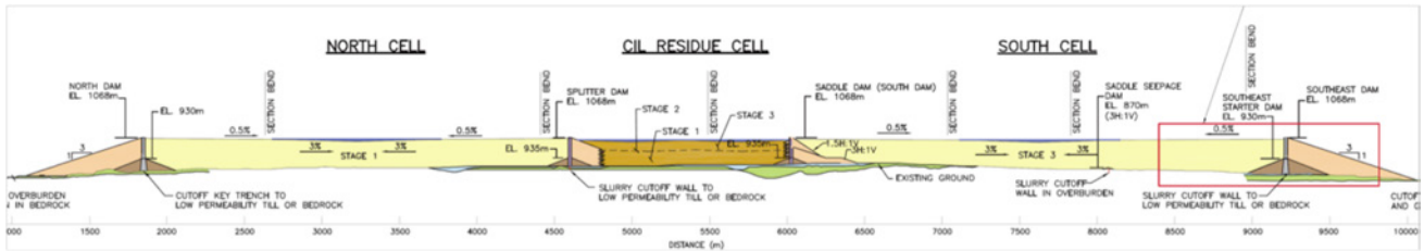
Figure 3 — KSM Tailings Impoundment Longitudinal Cross Section
