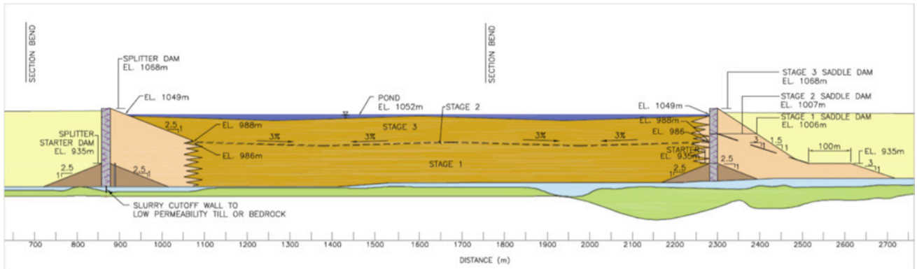
Figure 4 — KSM Lined Sulfide Residue Cell Cross Section
